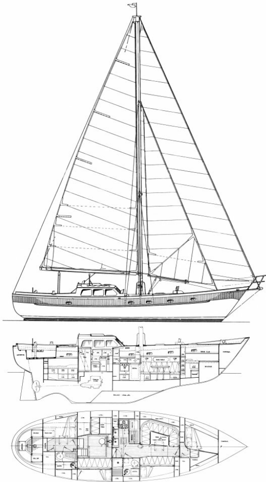
Pan Oceanic 46 Cutter
